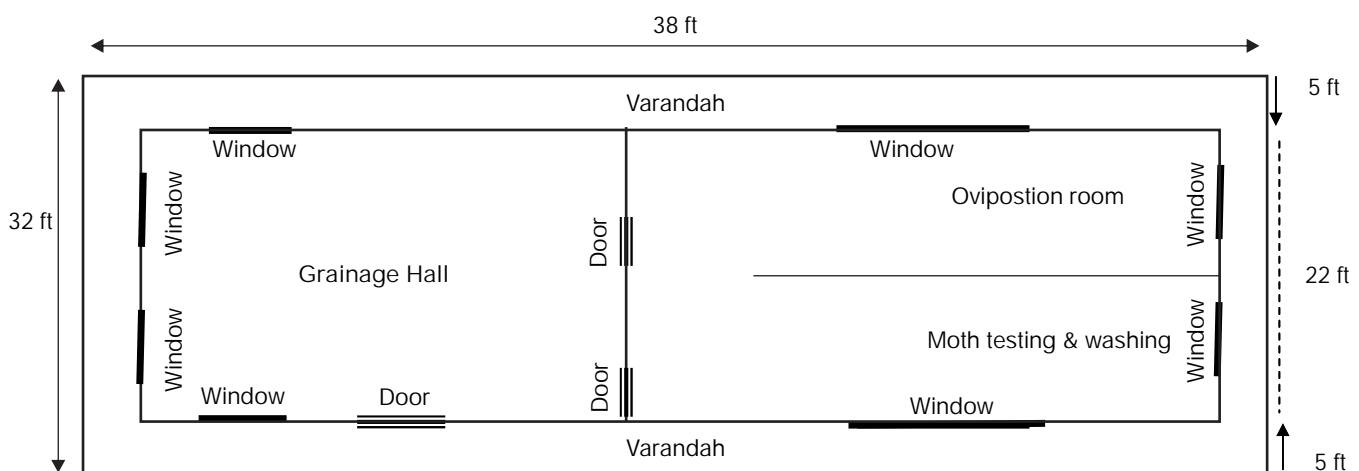
Indicative plan for Muga seed multiplication unit
